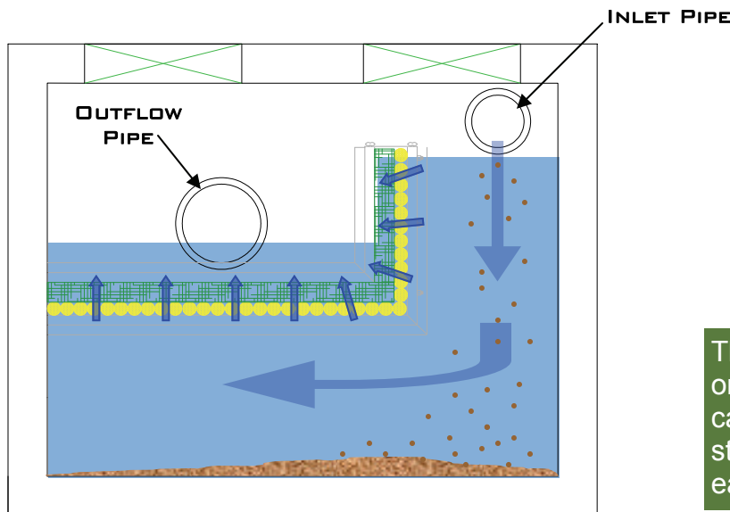
TREATMENT FLOW OPERATION
